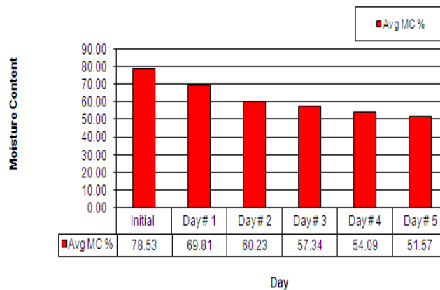
Figure 3: Typical moisture content A of Sun dried green material
