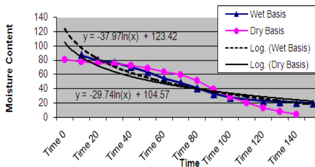
Figure 5: Comparison of Drying Characteristics
